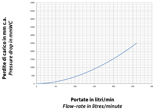
Scambiatore a fascio tubiero 3 m 2 Tube bundle heat exchanger 3 m 2
