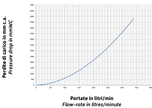
Scambiatore a fascio tubiero 8 m 2 Tube bundle heat exchanger 8 m 2
