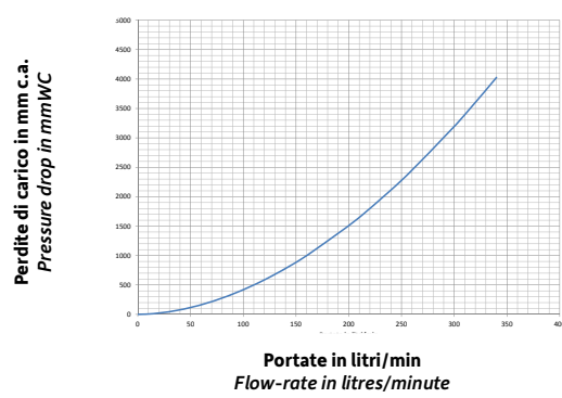
Scambiatore a fascio tubiero 6 m 2 Tube bundle heat exchanger 6 m 2
