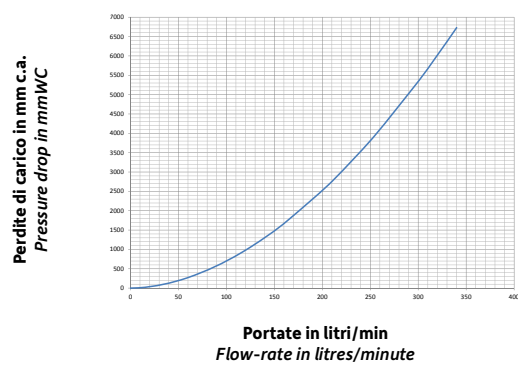
Scambiatore a fascio tubiero 10 m 2 Tube bundle heat exchanger 10 m 2
